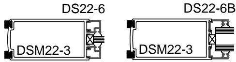
Optional Glass Stop for 1/4" or 1" Glass
