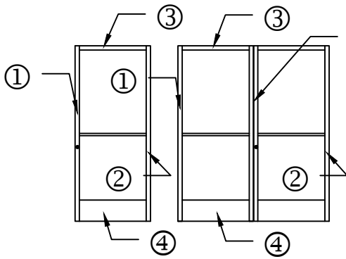
Optional Glass Stop for 1/4" or 1" Glass
