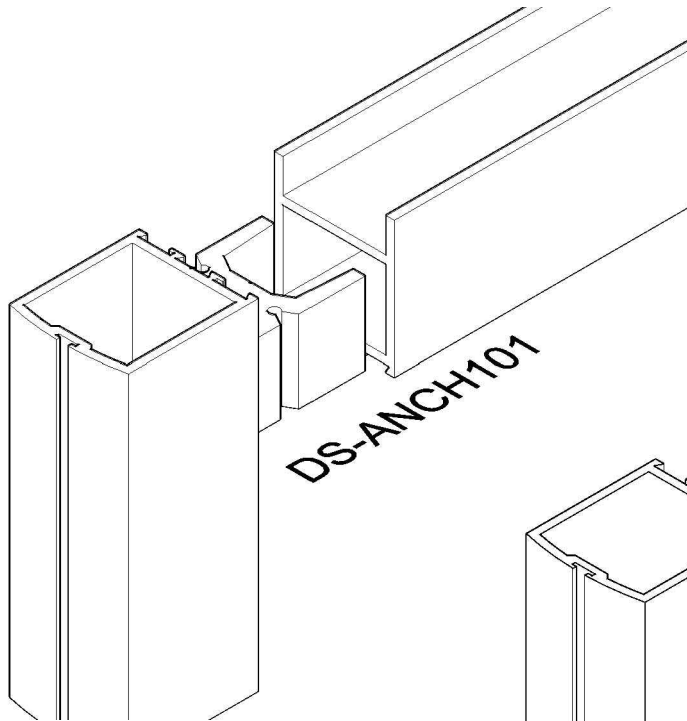
Joint of Door Stile & 2" Top Rail (Single Mohair)
