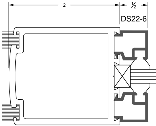
1/4" Glass Stop & Stile
