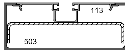
With 12 GA. Steel Stiffener
