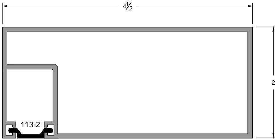
Pocket Filler
