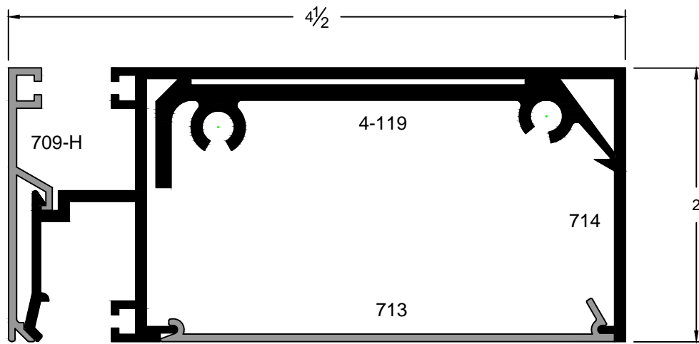
Horizontal Assembly
