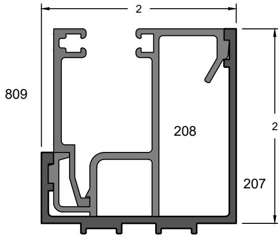
Sill Can Assembly
