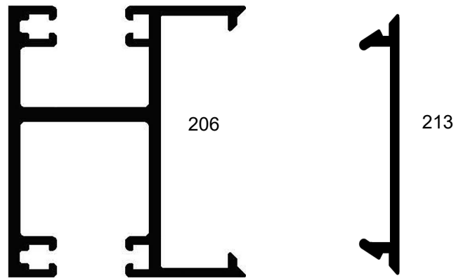
Inter. Vertical
