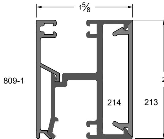
Horizontal Assembly
