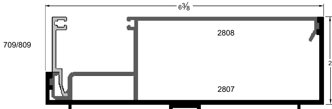
Sill Can Assembly
