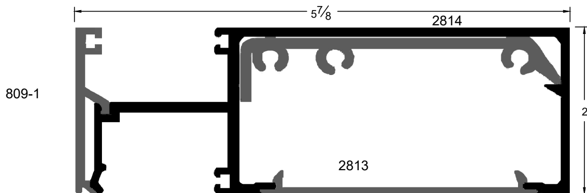
Horizontal Assembly
