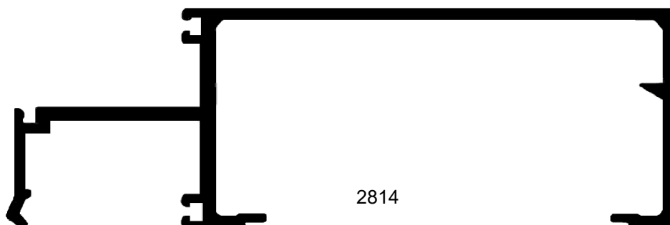
Horizontal w/ Screw
