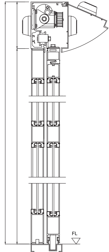
Side View
