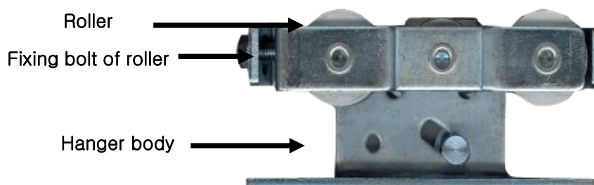
Hanger
