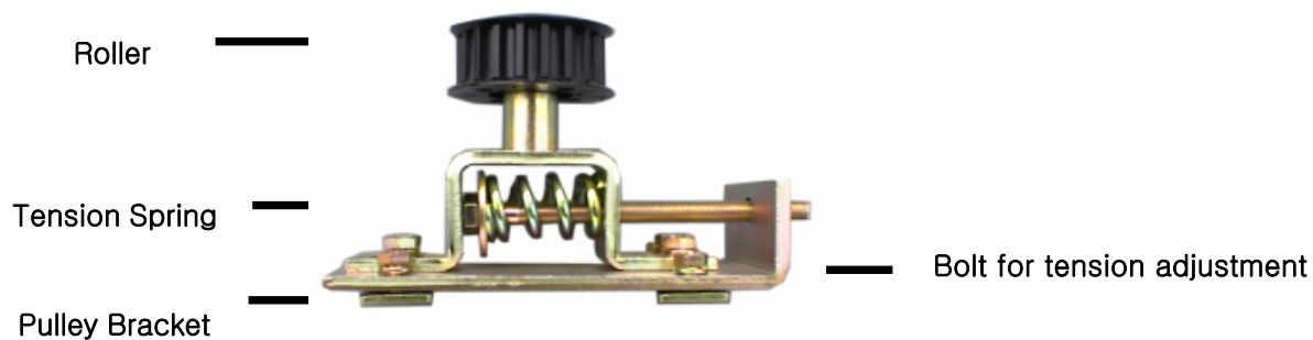
Driving Pulley
