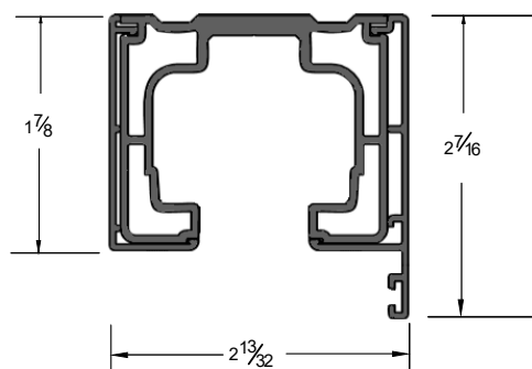
Top Track
