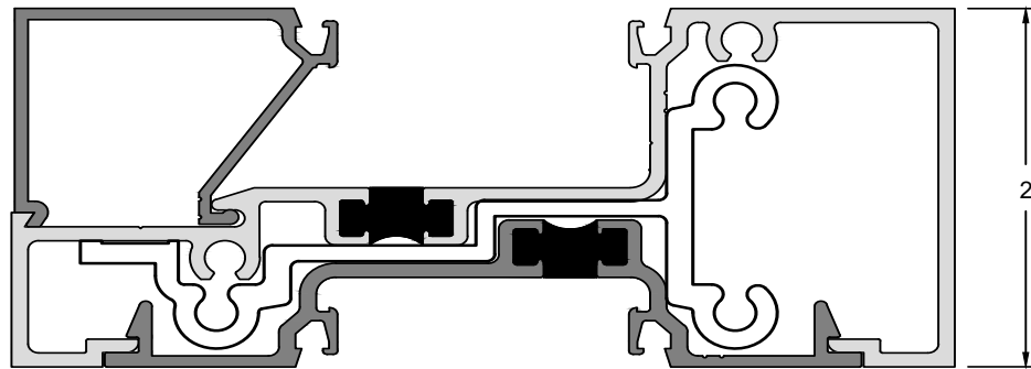
Horizontal Assembly
