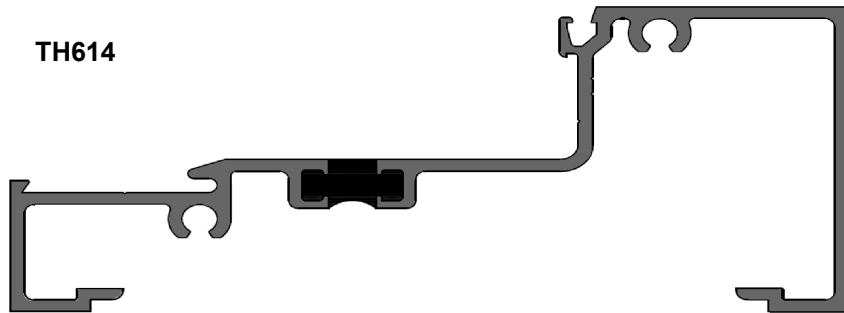
Horizontal
