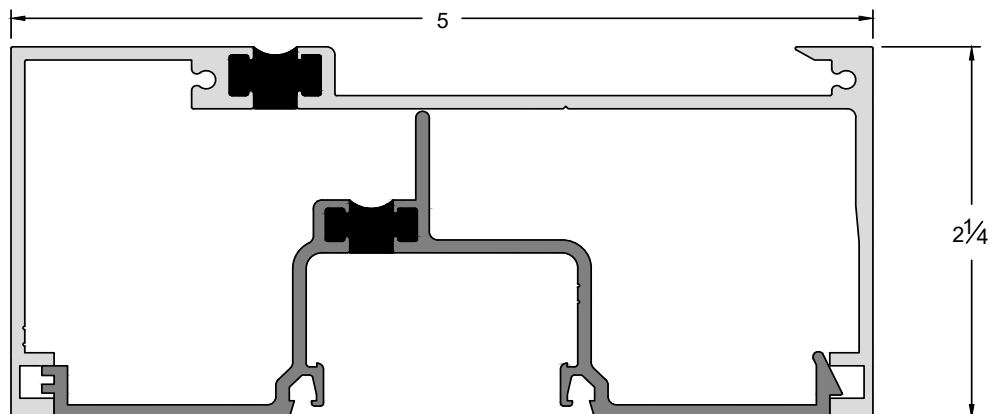
Horizontal Assembly
