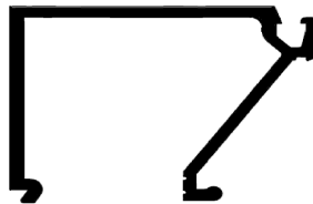
Glass Stop
