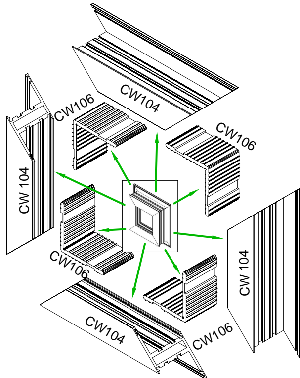
Inner Window
