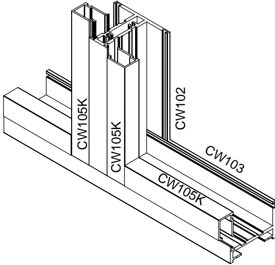
Installing Muntins
