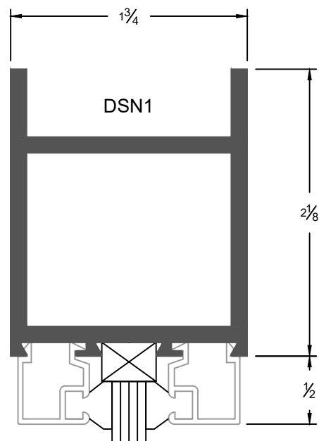
Top Rail
