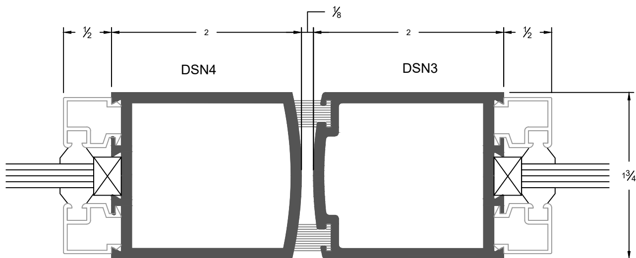
Meeting for Two Sliding Panels
