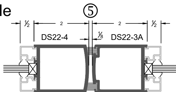
Meeting for Two Sliding Panels
