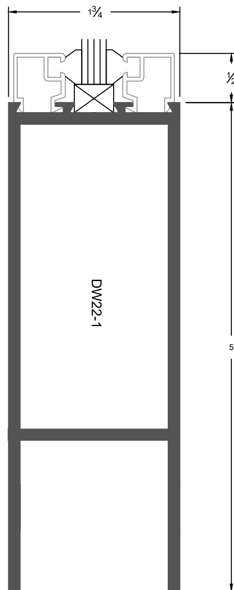
Bottom Rail
