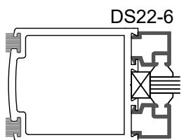
Optional Glass Stop for \frac{1}{4} " or 1" Glass
