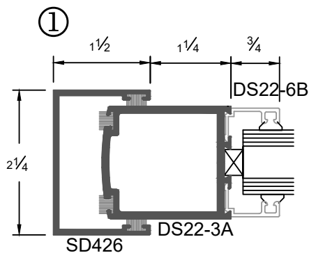
Fixed Panel
