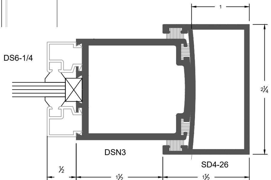
Sliding Panel
