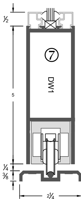
Top and Bottom Rails
