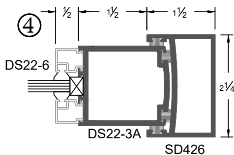
Sliding Panel
