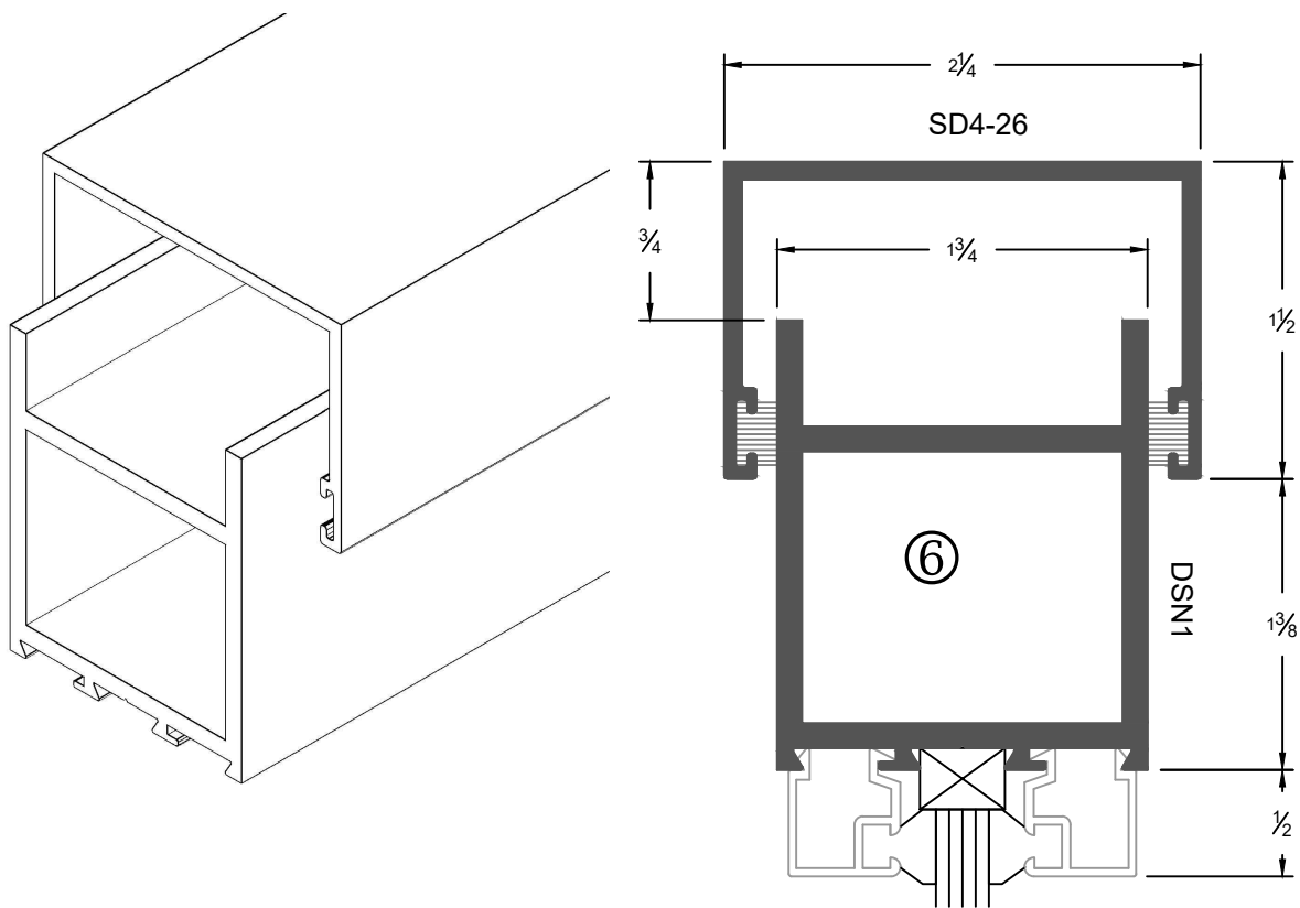
Top Track & Door Rail
