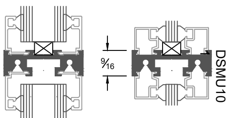
Optional Muntin ( \frac{9}{16} " up to 10")
