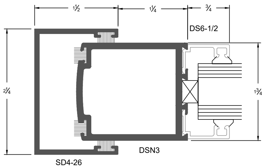
Fixed Panel
