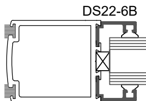
Optional Glass Stop for \frac{1}{4} " or 1" Glass
